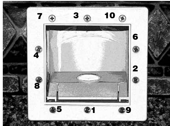
Skimmer faceplate installed with screw tightening sequence
