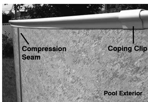
Premium 4" Coping
