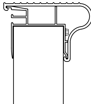
E. Plastic Aboveground Coping
